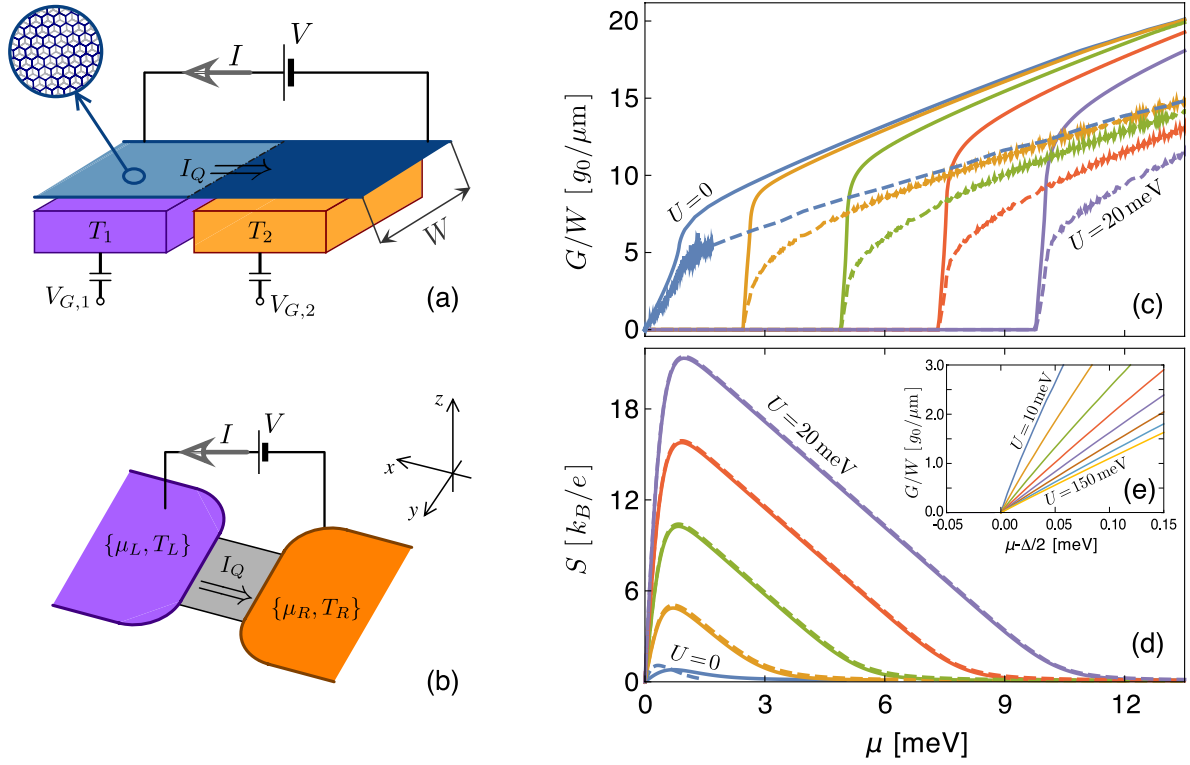
Figure 1. Systems studied numerically in the paper (left) and their basic thermoelectric characteristics (right). (a) BLG strip of width W with a voltage source driving electric current through the strip. Two gate electrodes, with different temperatures T_1 and T_2 , induce an abrupt interface (dash-dot line) between the weakly-doped (light area) and the heavily-doped (dark area) regions. (b) A finite, weakly-doped section of the strip (of length L ) with leads driving both thermal and electric currents. In both cases, additional gate electrodes (not shown) allow to tune the electrostatic bias between the layers (See footnote 1.). The coordinate system is also shown. (c) Zero-temperature conductance, specified in the units of g_0 = 4e^2/h , and (d) the Seebeck coefficient at T = 5 K as functions of the chemical potential. Solid lines correspond to the system of panel (a), dashed lines correspond to the system of panel (b). (e) Zoom-in of the conductance as a function of the chemical potential measured from the conduction band minimum ( \mu = \Delta/2 ) for the system of panel (a). Skew-interlayer hopping is fixed at t' = 0.3 eV. The electrostatic bias between the layers is varied from U = 0 to U = 20 meV in steps of 5 meV (c) and (d) or from U = 10 meV to U = 150 meV in steps of 20 meV (e). (The extreme values of U are specified for corresponding lines.)
