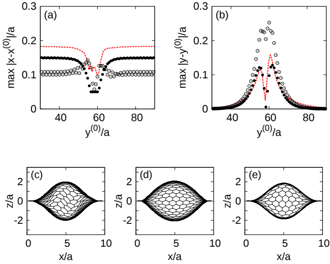
Figure 3: Spatial arrangement of carbon atoms after the optimization procedure presented in Sec. II B compared with the LAMMPS output. (a,b) Maximal displacement of an atom along (a) x -axis or (b) y -axis in the coordinate system of Fig. 1, after the optimization starting from initial coordinates x = x^{(0)} , y = y^{(0)} [see Eqs. (10), (11)]. Open (or closed) symbols correspond to \beta = 0 (or \beta = 3 ). Red dashed lines show the LAMMPS results for comparison [26, 27]. (c)–(e) C-C bonds after the optimization projected onto the x – z plane for (c) \beta = 0 , (d) \beta = 3 , and (e) the LAMMPS results. [Notice that difference in scales for x and z axes visually amplifies the buckling.] The system parameters are L = 90\sqrt{3}a , W = 11a , W'/W = 0.9 , and the kink position is y_0 = (3/8)L \approx 58.5a for all cases.
