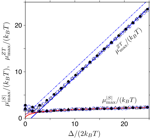
Figure 5. Chemical potential corresponding to the maximal absolute thermopower presented in figure 2 ( \mu_{\max}^S ) and the maximal figure of merit presented in figure 4 ( \mu_{\max}^{ZT} ) as function of the energy gap. Points correspond to same datasets as in figures 2(a) and (b) (skew-interlayer hopping integral is t' = 0.3 eV). Lines depict approximating equation (15) with \alpha = 1 (red solid line) and \alpha = 2 (red dash-dot line), equations (16) (blue solid line), and (17) (blue dash-dot line).
