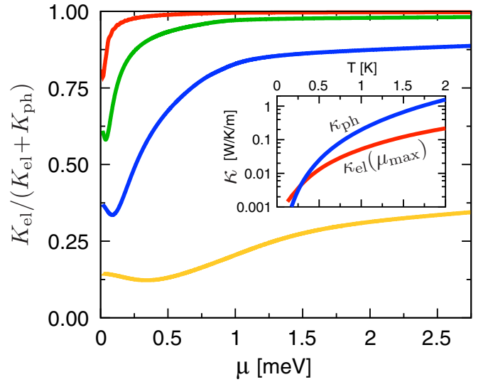
FIG. 6. Relative electronic contribution to the thermal conductance for t' = 0.3 eV as a function of the chemical potential. The temperatures are (top to bottom) T = 80 mK, 0.2 K, 0.515 K, and 2 K. Inset shows phononic [blue line] and electronic [red line] thermal conductivities ( \kappa = KL/(2dW) , with d = 0.335 nm the separation between layers) as functions of temperature, with the chemical potential fixed at \mu = \mu_{\max} corresponding to the maximal Seebeck coefficient.
