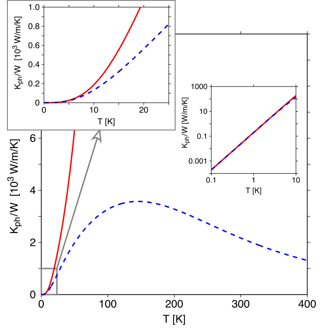
Figure 3. Phononic parts of the thermal conductance for the systems of figures 1(a) (solid line) and 1(b) (dashed line) as functions of temperature. Insets are zoom in, for low temperatures, in the linear (top left) and the log–log (right) scale.
