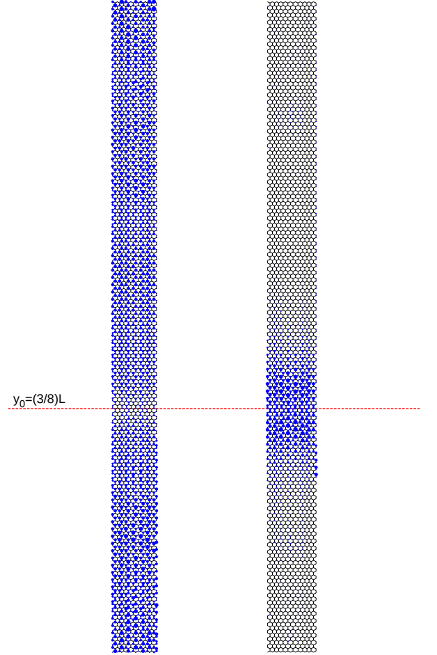
Figure 7: Local density of states for E = 0.04 t_0 for W = 10a (left) and W = 11a (right). Red horizontal line indicates the kink position. The bond lengths are optimized for \beta = 3 . Remaining system parameters are same as in Fig. 6.
