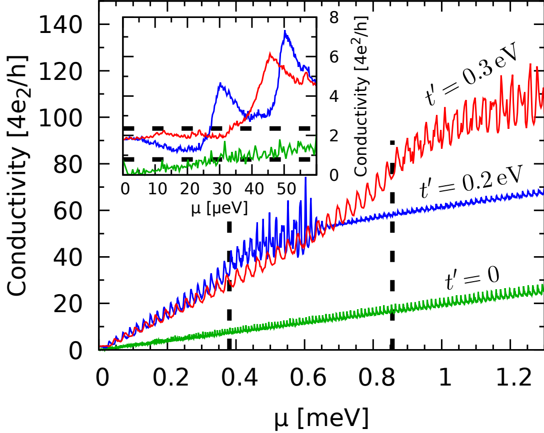
Figure 3: The zero temperature conductivity of bilayer graphene for 3 distinct values of trigonal warping (marked on picture). The vertical dashed lines corresponds to Lifshitz energies for considered values of trigonal warping (compare eq. 32). The inset is a zoom-in close to charge neutrality point. The horizontal lines corresponds to conductivities \sigma = 2\sigma_{\text{MLG}} = (8/\pi)e^2/h and \sigma = 6\sigma_{\text{MLG}} . Reprinted from [28].
