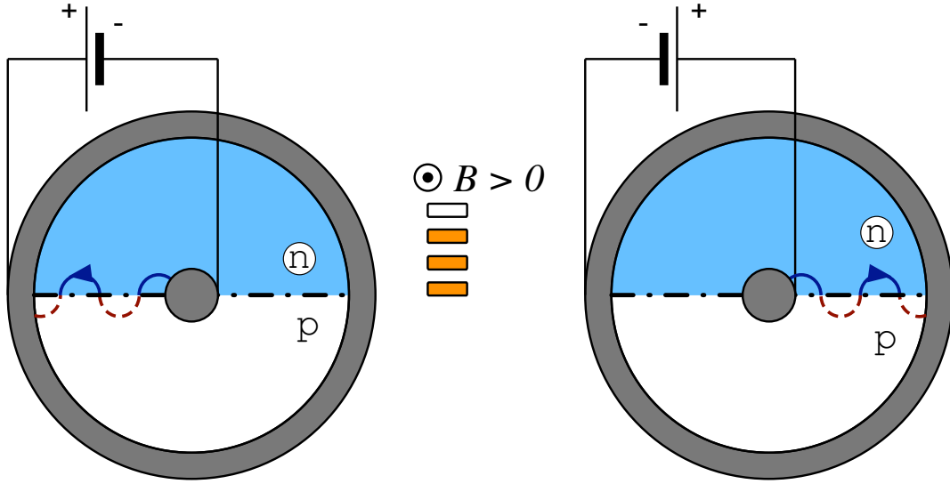
Figure 15: Quasiclassical picture of snake states. The electron (in n -doped region) traversing p-n junction changes into a hole (in p -doped region). This change is accompanied by change of sign of curvature radius. Reprinted from [51].
