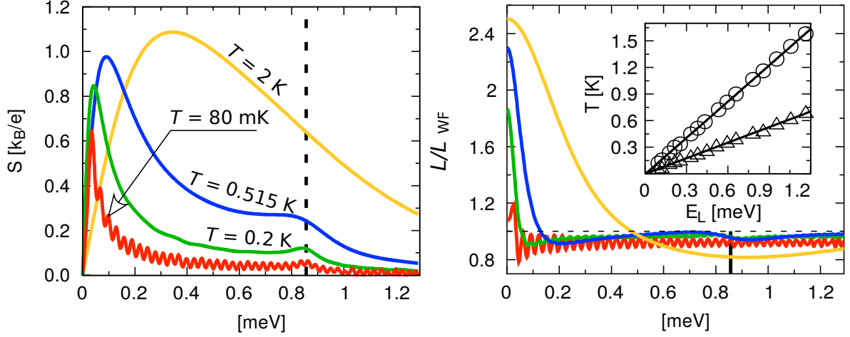
Figure 4: Left: The Seebeck coefficient for \gamma_3 = 0.3 eV for 4 different temperatures (see the picture). The dashed vertical line marks the Lifshitz energy. Right: The Lorentz number with respect to the value provided by Wiedemann-Franz law. The temperatures are the same as in the left panel. Inset shows the crossover temperature corresponding to disappearance of second maximum of Seebeck coefficient (triangles) and second minimum of Lorentz number (triangles) with respect to Lifshitz energy. Reprinted from [28].
